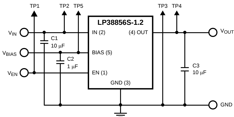
Figure 2. Evaluation Board Schematic
